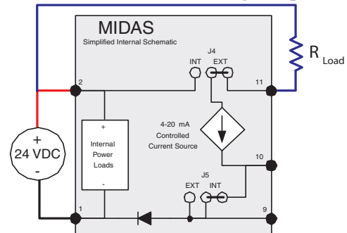
Diagram 4-9. Generic Example Midas® 3-Wire Sinking Output
