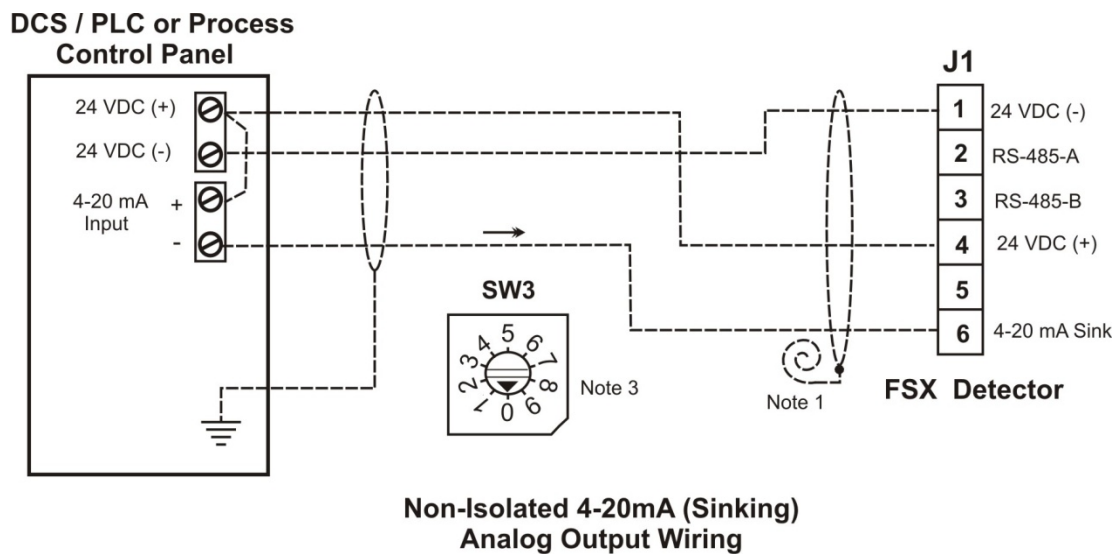
Figure 4-6 Typical Wiring for 4-20mA (Sinking) Analog Output
